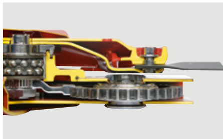
FAST-FIT ATTACHMENT : blades can be changed quickly.
